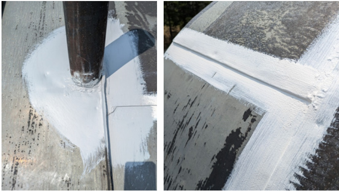
Sealing vulnerable areas using Hybrid Silicone Roof Patch
